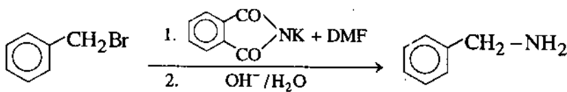
Benzyl bromua
