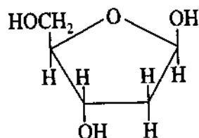
\beta -D-2-Deoxyribofuranozơ
