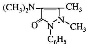
Piramidon
