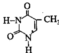
Timin
