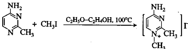
4-Amino-1,2-dimetyl-1-pirimidini iodua
