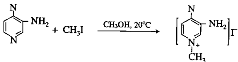
2-Amino-4-metyl-4-pirazini iodua
