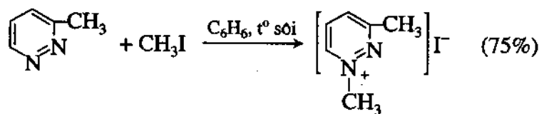
3-Methylpiridazin
